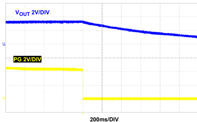
FIGURE 48. OVER-TEMPERATURE PROTECTION
