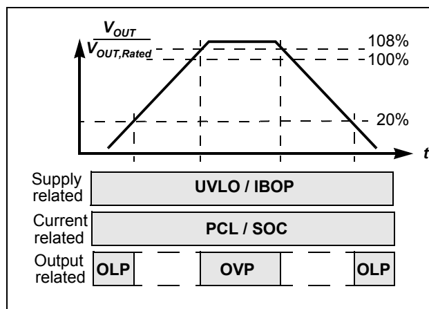
Figure 6 Protection Features
